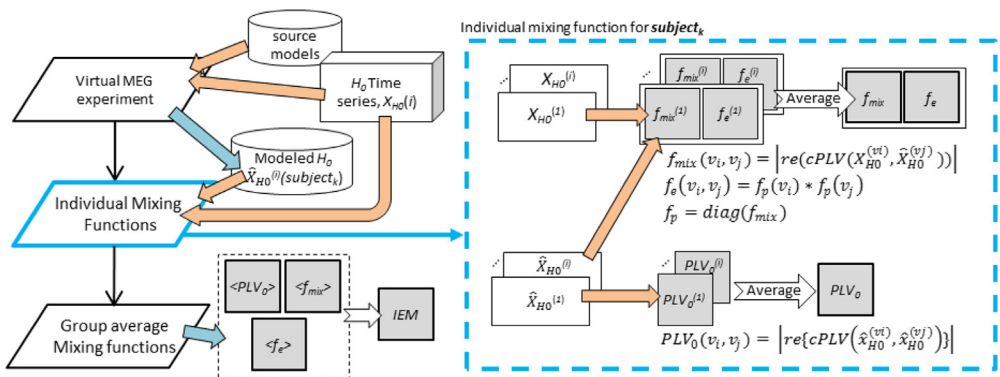
Fig. 5. The workflow for computing the mixing properties. IEM: group-level intractable-edge-mask. PLV_c : the residual spread function. f_{mix} : the mixing function. f_e : the edge fidelity function.
